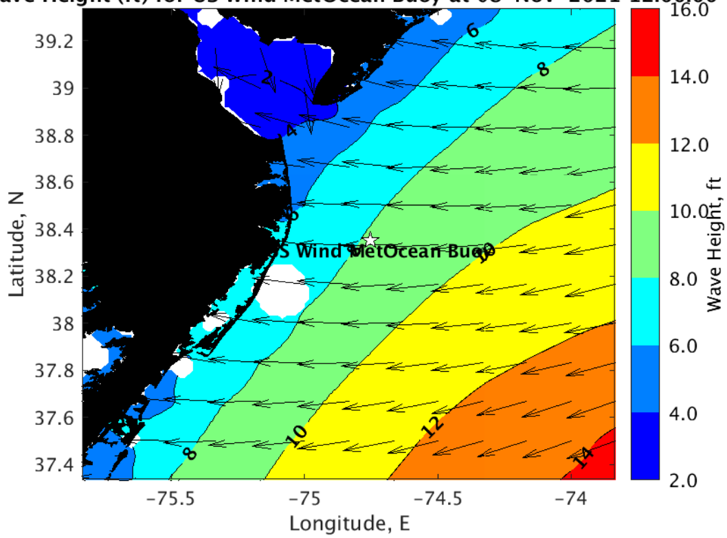
Wave Height (ft) for US Wind MetOcean Buoy at 08-Nov-2021 12:00:00
