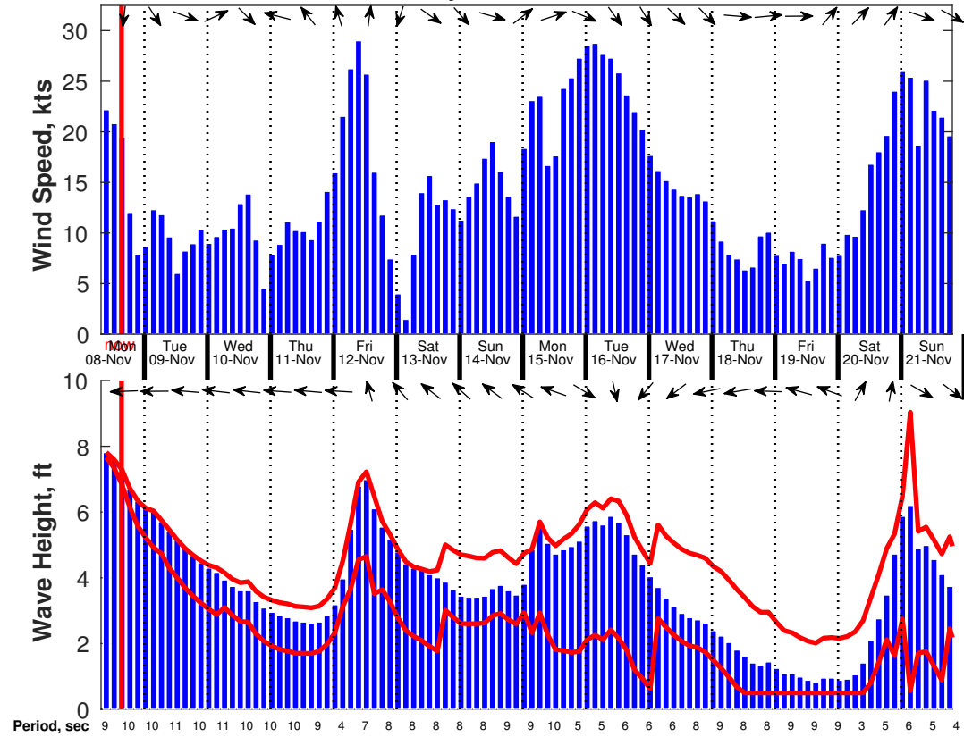
Wind & Wave Forecast for US Wind MetOcean Buoy from 08-Nov-2021 08:00:00 to 22-Nov-2021 02:00:00
