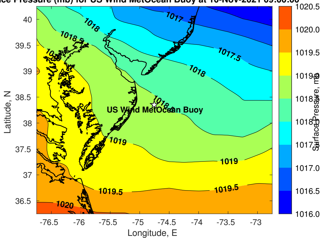
Surface Pressure (mb) for US Wind MetOcean Buoy at 10-Nov-2021 09:00:00
