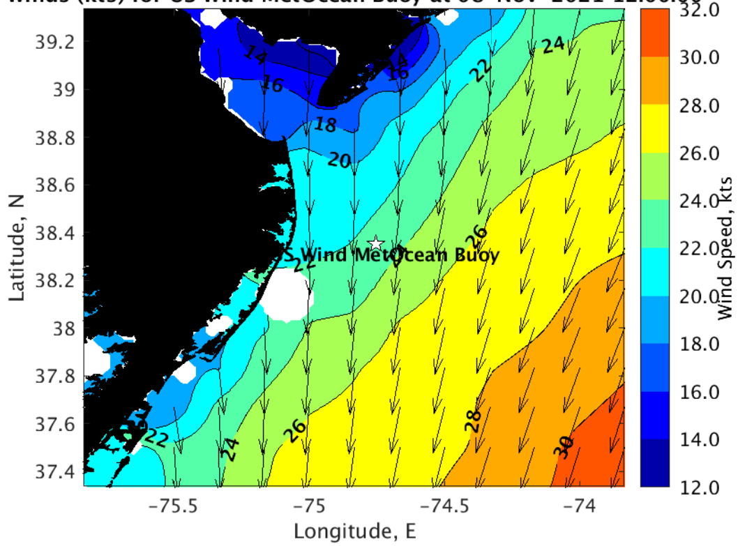
Winds (kts) for US Wind MetOcean Buoy at 08-Nov-2021 12:00:00
