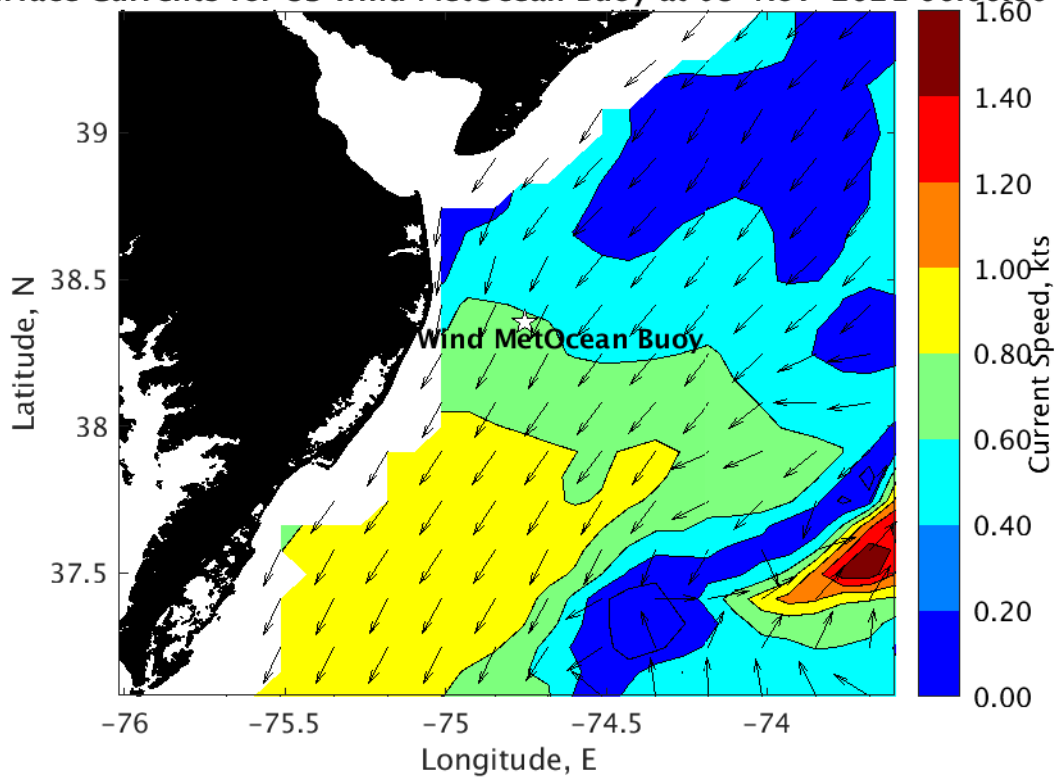
Surface Currents for US Wind MetOcean Buoy at 08-Nov-2021 00:00:00
